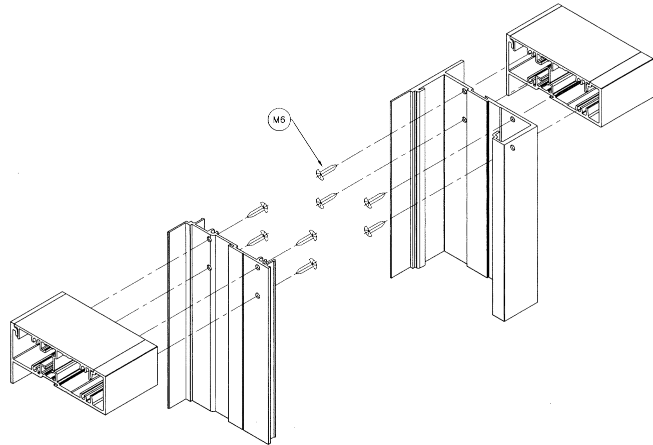
MULLION CORNER
